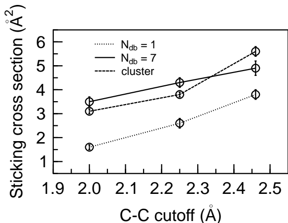
FIG. 3. Sticking cross sections obtained using the classical Brenner hydrocarbon potential for the cases with one dangling bond on the surface ( N_{db} = 1 ), seven dangling bonds on the surface ( N_{db} = 7 ), and one dangling bond on top of a cluster (cluster), consisting of four carbon atoms (three of these saturated). The methyl gas temperature was in all the cases 2100 K.
