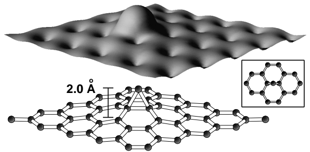
FIG. 3. Atomic and electronic structure of the D3 defect identified in our simulations. The constant-value surface corresponds to a valence electron density of 0.02 e/\text{bohr}^3 . To provide a clear view of the atomic structure, the electron density has been raised in the figure. The inset shows the defect viewed from above the graphite (1000) surface.
