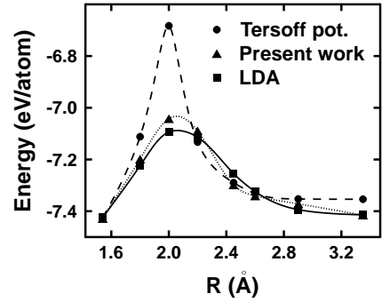
FIG. 2. Total energy per atom of the diamond to rhombohedral graphite transformation as a function of the interlayer distance R parameter. The squares show the energy given by ab initio calculations in Ref. [22], the circles the result of the original Tersoff potential, and the triangles the result of our potential. The lines are drawn to guide the eye.
