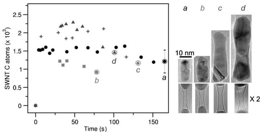
Figure 4. Estimated number of carbon atoms in SWNTs grown from four different Co particles as a function of time (assuming a SWNT surface density of 38.3 \text{ carbon atoms nm}^{-2} ). The points enclosed in circles mark SWNT rupture. The labels a–d indicate from which particle the data points were taken. The volumes of the starting metal particles were 0.7 (a), 1.3 (b), 3.1 (c) and 6.1 (d) \times 10^3 \text{ nm}^3 , respectively. The TEM was operated at 200 kV and the sample temperature was kept at 600 °C. Images of the starting Co particles as well as the SWNTs grown from them are shown on the right-hand side. Since the growth was too rapid to be monitored in detail, the growth speed cannot be extracted from the slopes of the curves (the first data points of the curves had to be taken at different times due to technical reasons).
