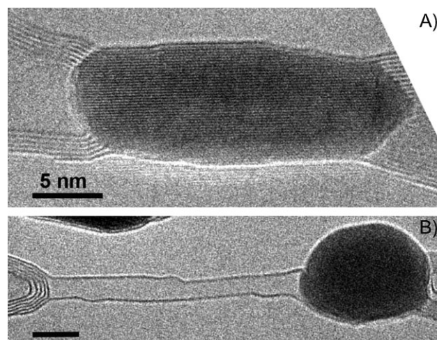
Figure 2. Growth of a SWNT at a MWNT–Co interface. The sample was irradiated with 200 keV electrons at 700 °C. A) MWNT–Co–MWNT heterojunction. The Co particle is in the crystalline state and the graphitic layers of the tube are directly connected to the metal lattice without a graphitic surface layer on the metal. B) After irradiating the interface between the MWNT on the left-hand side and the Co particle for 18 min with an intense beam, the metal particle detached and retracted from the MWNT and transformed to a spherical shape. During this process, a SWNT grew and bridged the gap between the Co particle and the MWNT. Scale bar: 5 nm.
